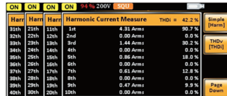
Current Harmonic
