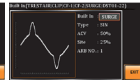
SURGE Waveform
