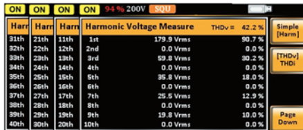
Voltage Harmonic
